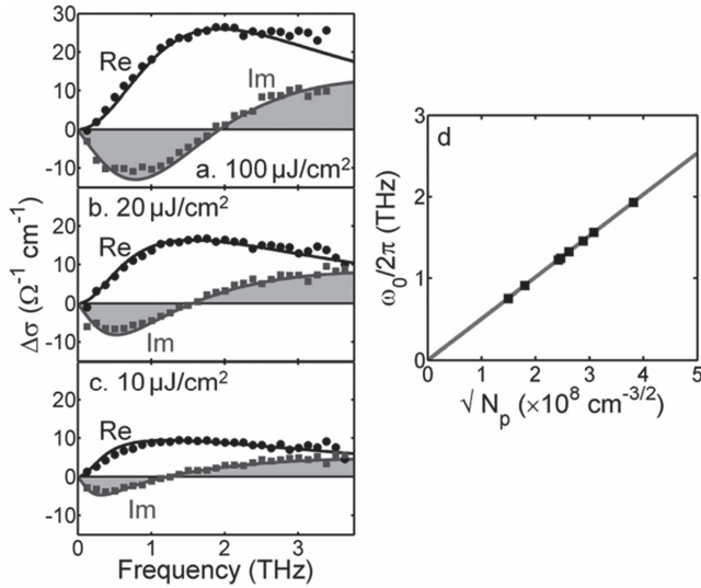
Figure 13. Dependence of photoconductivity spectra on carrier density in GaAs nanowires. The photoconductivity spectra were obtained 2 ps after photoexcitation at fluences of (a) 100, (b) 20 and (c) 10 \mu\text{J cm}^{-2} . Spectra were fitted with the surface plasmon model. At the resonant frequency \omega_0 , the real part of \Delta\sigma(\omega) reaches a maximum and the imaginary part of \Delta\sigma(\omega) is zero. The charge carrier density increases with increasing fluence, accompanied by a shift in the resonant frequency \omega_0 . (d) Surface plasmon resonance frequencies \omega_0 versus the square root of the photoexcited carrier density N_p . Reprinted with permission from [51]. Copyright 2013 Institute of Physics.
