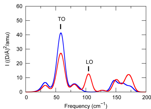
Figure 10. Calculated infrared absorption intensities of MAPbI 3 in the low-temperature orthorhombic phase corresponding to the TO modes (blue line) and to the LO modes (red line). For clarity, only the frequency region with the largest LO–TO splitting is shown. The black bars indicate the LO–TO doublet discussed in section 4.2. The infrared activities of the LO modes are calculated for a wavevector along the [111] direction.
