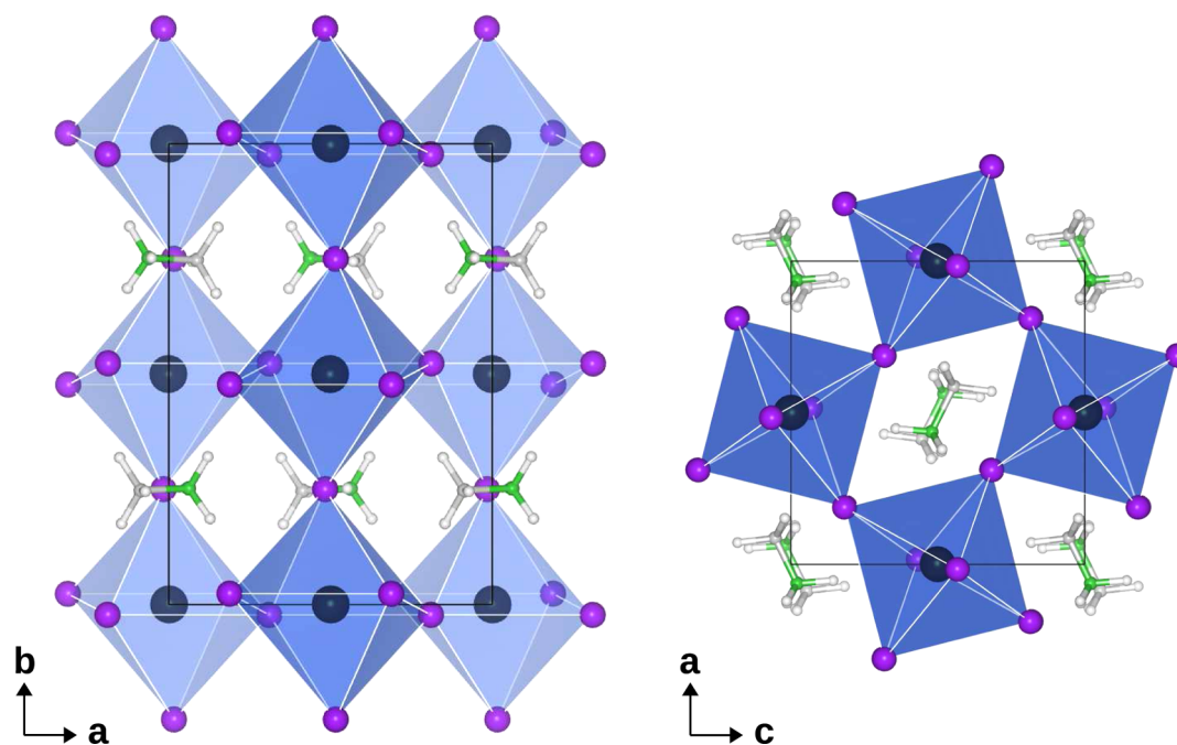
Figure 1. Optimized structure of MAPbI 3 in the orthorhombic phase. The Pb atoms are represented by the large black spheres in the center of the shaded octahedra. The smaller purple spheres located at the corners of the octahedra indicate the I atoms. The MA cations are represented using ball-and-stick models, with gray, green, and white spheres denoting C, N, and H atoms, respectively. The unit cell is indicated by the black straight lines, with the axes given at the bottom.
