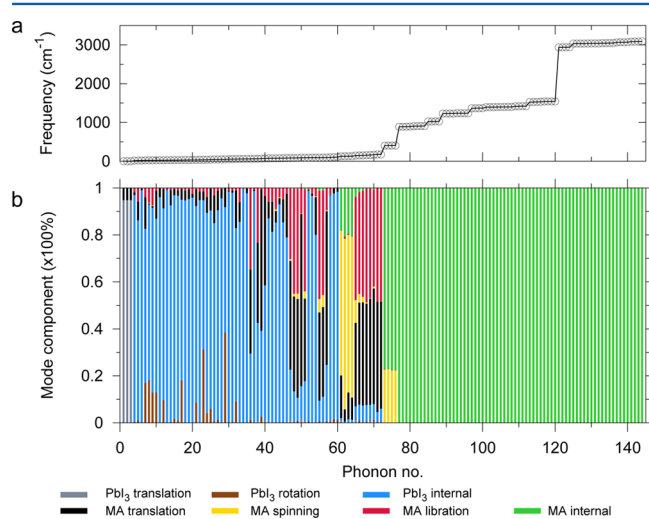
Figure 2. (a) Calculated vibrational frequencies for each eigenmode (discs). The line is a guide to the eye. (b) Decomposition of the vibrational modes of \text{MAPbI}_3 in the low-temperature orthorhombic phase at the \Gamma point. The height of each stick represents the contribution of the corresponding vibration to each eigenmode, according to eq 6. The color code is indicated in the legend.
